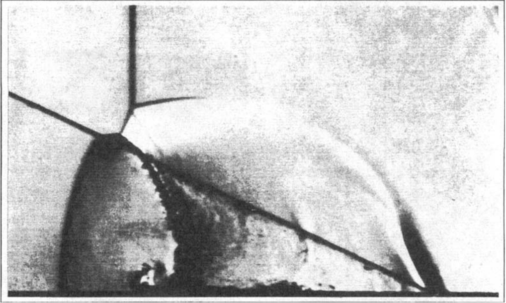
FIGURE 9. (a) Schlieren photograph and (b, c) colour contour plots for a twin Mach reflection type refraction, TMR (see figure 2f), with \xi_i = 0.18 and \alpha_i = 66^\circ at a \text{CO}_2/\text{CH}_4 gas interface.
