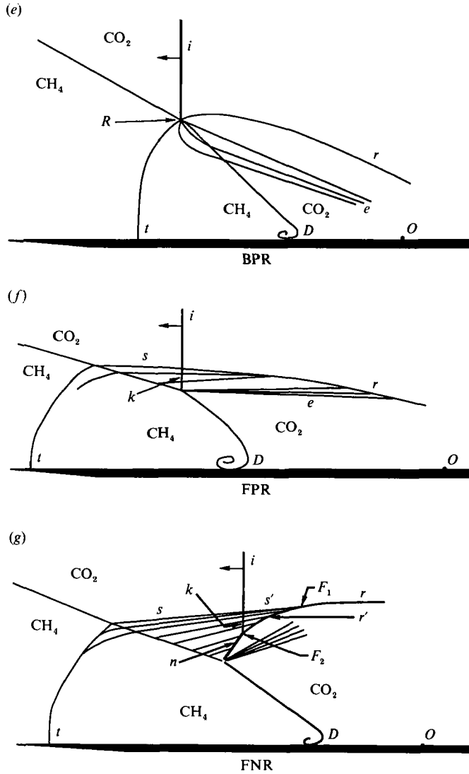
FIGURE 3. Polar diagrams for a weak shock refraction sequence with \xi_t = 0.78 at a pure \text{CO}_2/\text{CH}_4 gas interface. (a-c) Regular refraction, (d) transition, and (e-g) irregular refraction. (a) Reflected expansion, RRE, at \alpha_i = 27^\circ , |Z_i| < |Z_t| ; (b) degenerate refraction at the angle of intromission \alpha_i = \alpha_{im} \approx 32.0592^\circ , Z_t = Z_i , R = 0 , T = 1 , the condition for total energy transmission; (c) reflected shock, RRR, at \alpha_i = 33.27^\circ , |Z_t| > |Z_i| ; (d) the shock critical angle \alpha_{sc} \approx 34.4885^\circ ; (e) bound precursor refraction, BPR, \alpha_i > \alpha_{sc} ; (f) free precursor refraction, FPR, s and t are evanescent waves; (g) free precursor refraction with Neumann refraction, FNR, M_{oi} , M_{ot} , M_{or} , free-stream Mach numbers upstream, and relative to the i , t , and r shocks respectively; (\epsilon_1, \lambda_1, \lambda_2) solutions of the von Neumann regular refraction theory; D , disturbed gas interface; A_1 , intersection point of the primary polars ( i, t ). For other symbols see the caption to figure 2.
