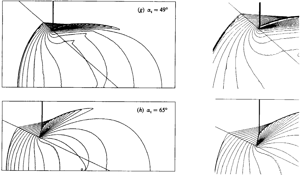
FIGURE 4. Contour plots of \log P for a weak shock refraction sequence with \xi_i = 0.78 at a pure \text{CO}_2/\text{CH}_4 gas interface. (a) \alpha_i = 27^\circ , RRE; (b) total transmission at the angle of intromission, \alpha_i = \alpha_{im} \approx 32.0592^\circ ; (c) \alpha_i = 33.27^\circ , RRR; (d) \text{RRR} \rightleftharpoons \text{BPR} , \lambda_1 \equiv \lambda_2 , at the shock critical angle \alpha_{sc} \approx 34.4885^\circ ; (e) \alpha_i = 38^\circ , BPR; (f) \alpha_i = 43^\circ , FPR; (g) \alpha_i = 49^\circ , FPR; (h) \alpha_i = 65^\circ , FNR. (The straight line running diagonally from upper left to lower right represents the initial, undisturbed gas interface. It is not a pressure contour.)
