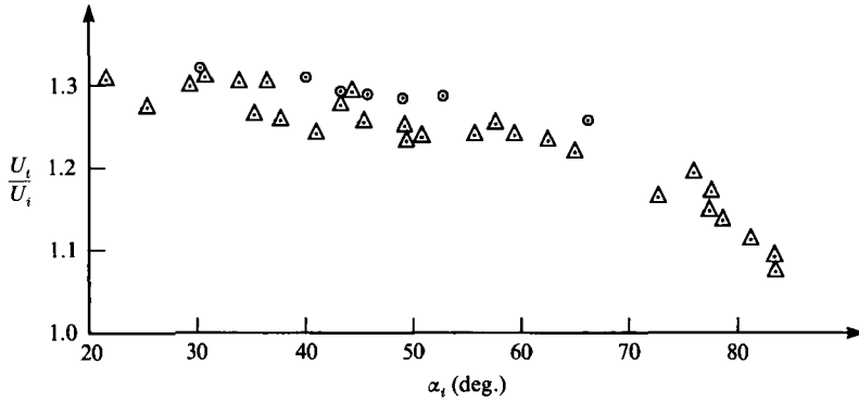
FIGURE 11. Comparison of the wave speed ratio U_t/U_i (see figure 2c) for a \text{CO}_2/\text{CH}_4 gas interface with \xi_t = 0.18 . \odot , Computed data for pure gases; \triangle , experimental data (from Abd-El-Fattah & Henderson 1978b).
