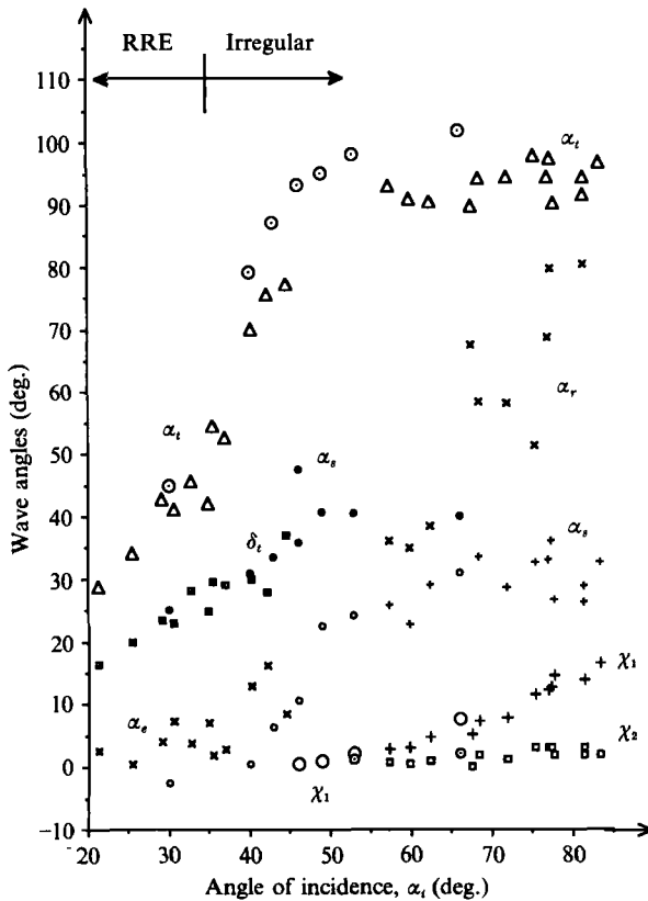
FIGURE 12. Experimental and computational wave angle data for a \text{CO}_2/\text{CH}_4 refraction with \xi_t = 0.18 . Circular symbols represent data from computations with pure gases. All other symbols represent experimental data. \odot , \triangle , Transmitted shock angle \alpha_t ; \circ , \times , reflected wave angle \alpha_r or \alpha_r ; \bullet , + , side shock angle \alpha_s ; \odot , \square , interface deflection angle \delta_t ; \circ , + , trajectory path angle \chi_1 ; \odot , \square , trajectory path angle \chi_2 . (Experimental data from Abd-El-Fattah & Henderson 1978b.)
