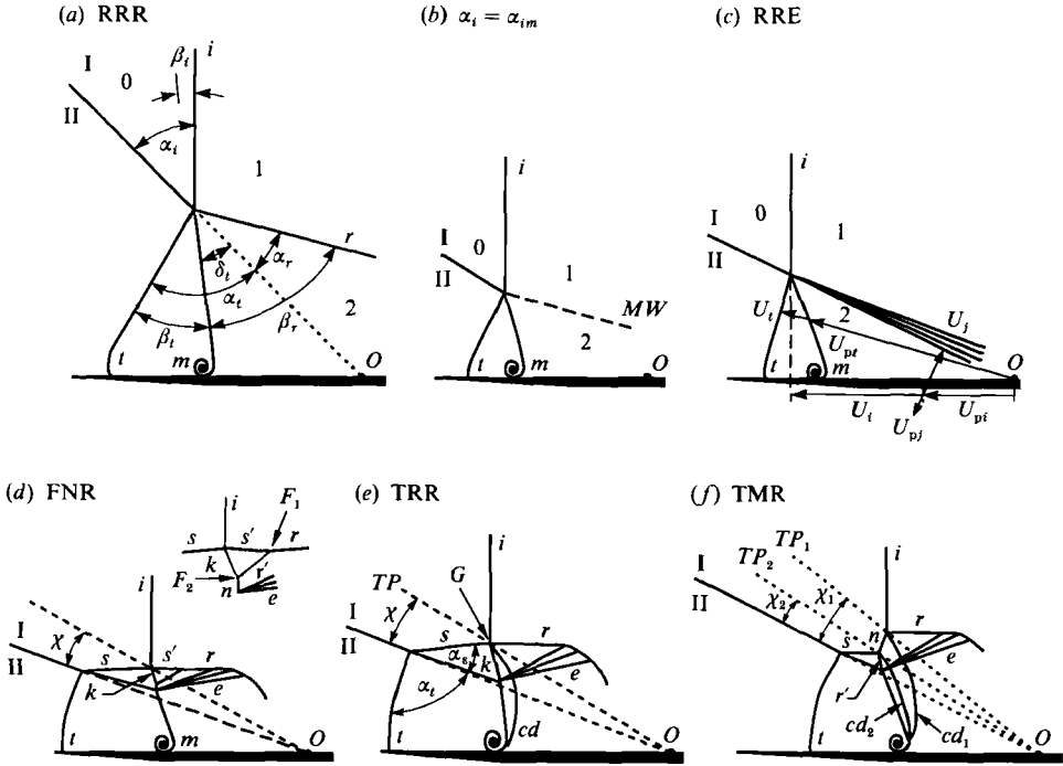
FIGURE 2. (a-c) Regular and (d-f) irregular shock refraction systems for a slow-fast \text{CO}_2/\text{CH}_4 gas interface, n < 1 . (a) Reflected shock, RRR, |Z_i| > |Z_t| , \alpha_t > \alpha_i ; (b) reflected Mach line degeneracy, |Z_i| = |Z_t| , \alpha_t = \alpha_i = \alpha_{im} ; (c) reflected expansion, RRE, |Z_i| < |Z_t| , \alpha_t > \alpha_i ; (d) free precursor von Neumann refraction, FNR; (e) twin regular reflection-refraction, TRR; (f) twin Mach reflection-refraction, TMR. i , Incident shock; t , transmitted shock; r , r' , reflected shocks; e , reflected expansion wave; k , modified incident shock; n Mach shock; s , side shock; s' , modified side shock; m gas interface; I, Region of undisturbed \text{CO}_2 ; II, region of undisturbed \text{CH}_4 ; MW , Mach line; cd_{(1,2)} , contact discontinuity; TP_{(1,2)} , trajectory path of shock wave confluences; \chi_{(1,2)} , trajectory path angles of shock wave confluences; F_{1,2} , shock triple points; G , quadruple point; O origin where i first encountered gas interface.
