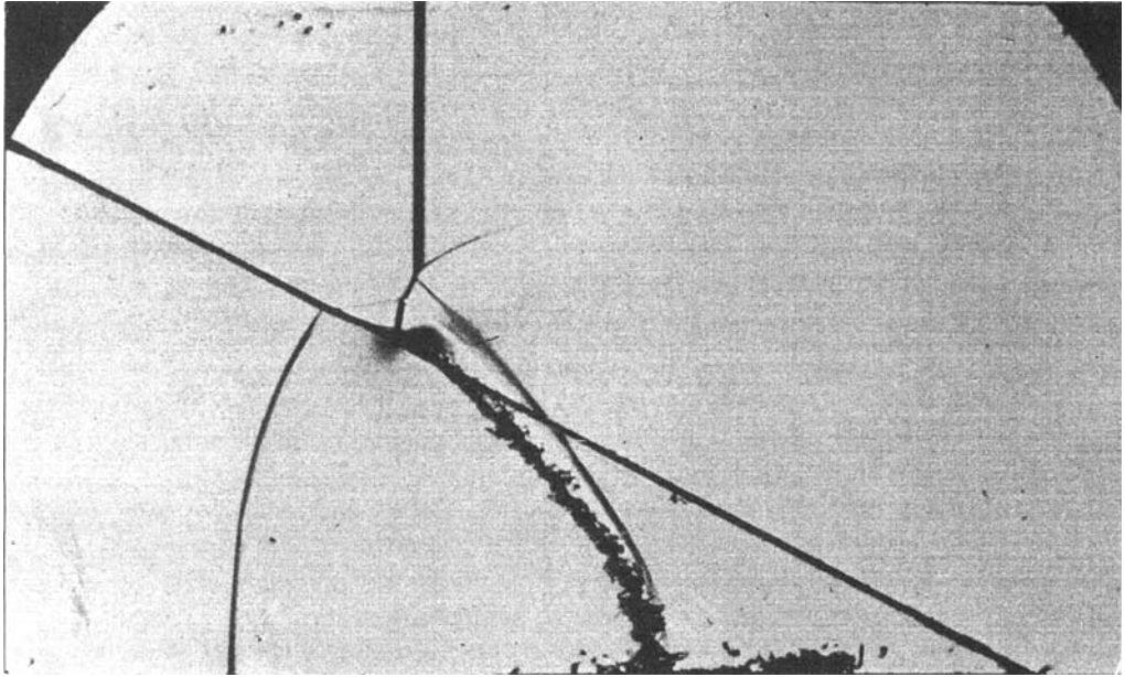
FIGURE 14. (a) Schlieren photograph and (b, c) colour contour plots for a twin von Neumann irregular refraction, TNR (Abd-El-Fattah & Henderson 1978 b ) at a \text{CO}_2/\text{CH}_4 gas interface with \xi_i = 0.53 and \alpha_i = 62^\circ .
