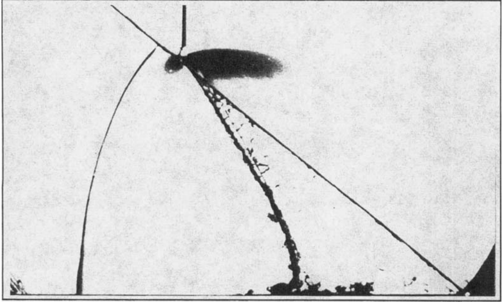
FIGURE 13. (a) Schlieren photograph and (b, c) colour contour plots for a twin regular reflection type refraction, TRR (see figure 2e) \xi_i = 0.53 , \alpha_i = 50.5^\circ , at a \text{CO}_2/\text{CH}_4 gas interface. See also the caption to figure 5.
