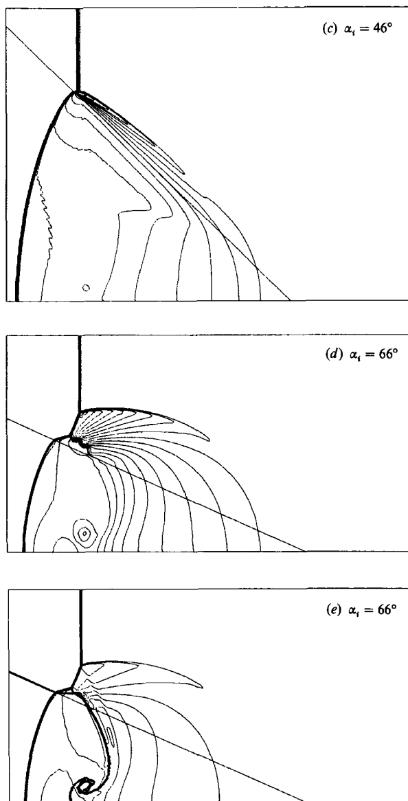
FIGURE 8. Contour plots of (a-d) \log P and (e) \log \rho from computations of a strong shock refraction sequence, \xi_i = 0.18 , at a pure \text{CO}_2/\text{CH}_4 gas interface. (The straight line running diagonally from upper left to lower right represents the initial, undisturbed gas interface. It is not a pressure contour.)
